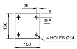
BASE PLATE 150 x 150 x 5 THK.
