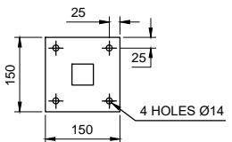
STANDARD POST WITH BASE PLATE 150 x 150 x 5 THK.
