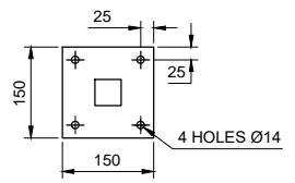
OFFSET POST WITH BASE PLATE 150 x 150 x 5 THK.
