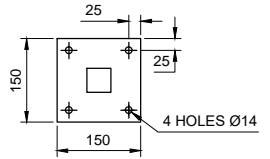
CORNER POST WITH BASE PLATE 150 x 150 x 5 THK.
