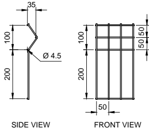
SIDE VIEW FRONT VIEW UNICO MESH DETAILS
